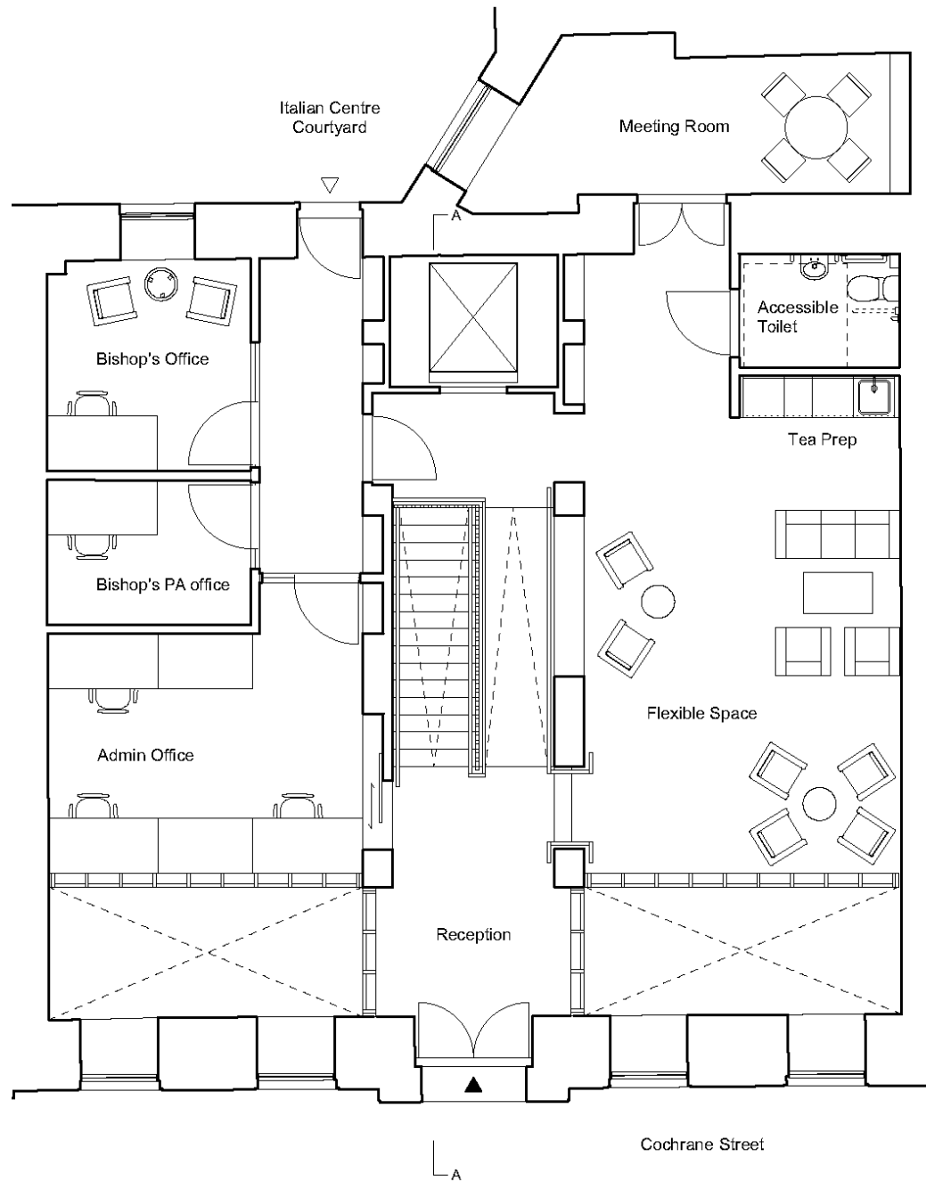
Ground Floor Plan as Proposed Scale: 1:100
